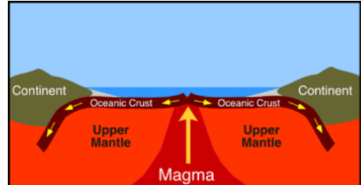
Picture from http://www.eoearth.org/image/Seafloor_spreading_diagram.gif
