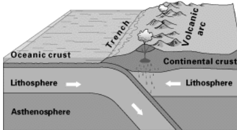
Oceanic-continental convergence
