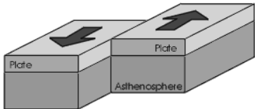
Transform
